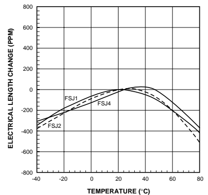
Figure 3 – Electrical Length Change vs. Temperature FSJ1-50A, FSJ2-50, FSJ4-50B
