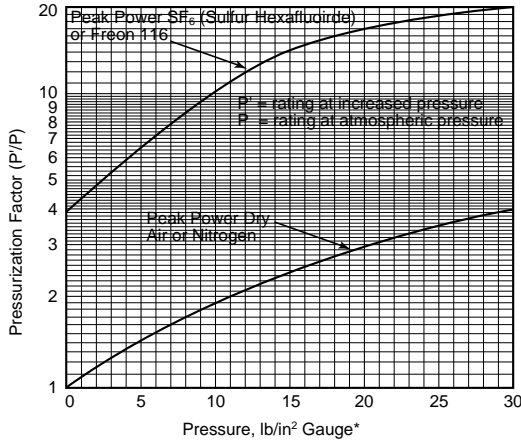
Figure 3 – Pressurization Factors
