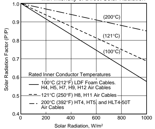
Figure 6 – Variation of Average Power Rating with Intensity of Direct Solar Radiation
