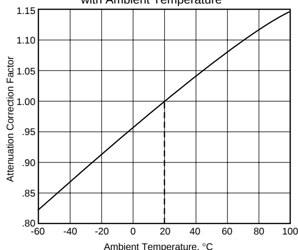
Figure 1 – Variation of Attenuation with Ambient Temperature
