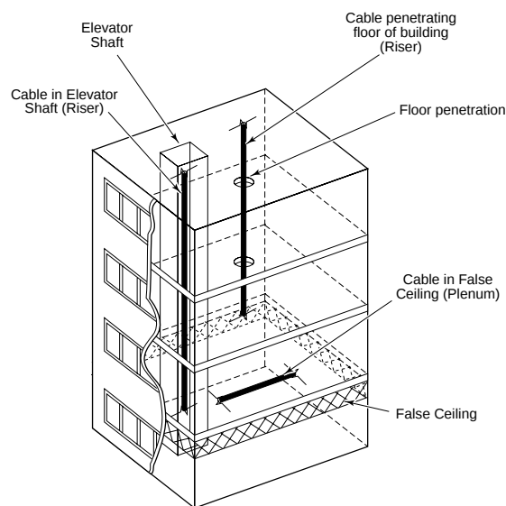
Riser and Plenum Applications in Multi-Story Building
