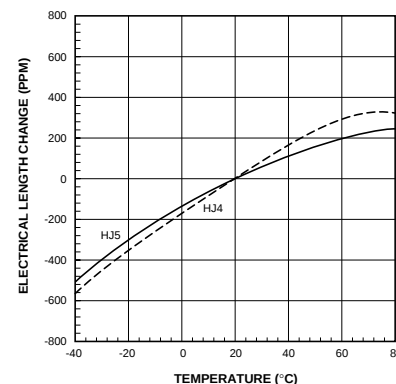
Figure 6 – Electrical Length Change vs. Temperature HJ4-50, HJ5-50
