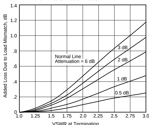
Figure 2 – Effect of Load VSWR on Transmission Loss
