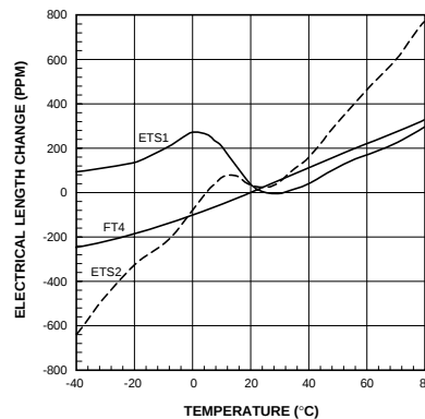
Figure 5 – Electrical Length Change vs. Temperature ETS1-50, ETS2-50, FT4-50
