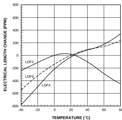
Figure 4 – Electrical Length Change vs. Temperature LDF1-50, LDF2-50, LDF4-50A, LDF5-50A
