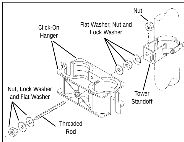
Round Adapter Attachment
